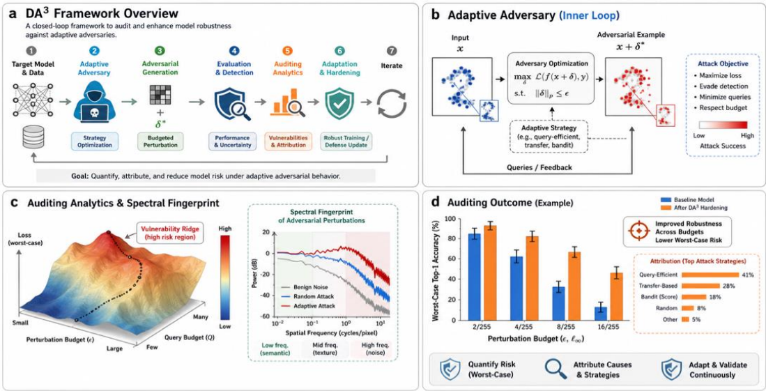
Fig 1: D3 Framework.
