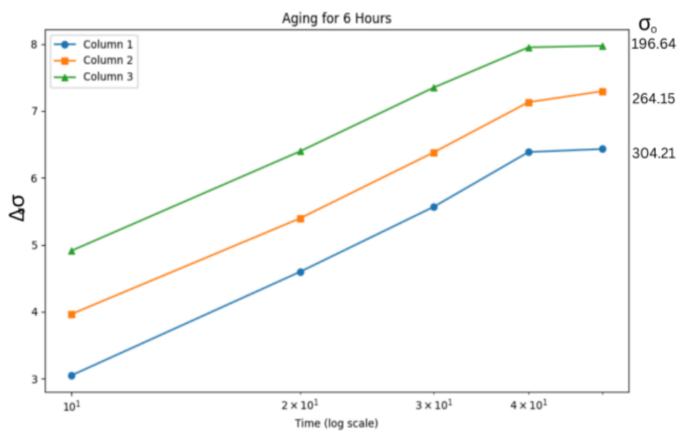
Figure 3.4 Alloy's Response to Stress Relaxation with 6 Hours of Aging.
