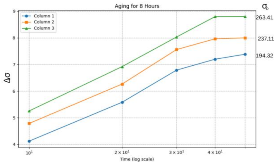
Figure 3.5 Alloy's Response to Stress Relaxation with 8 Hours of Aging
